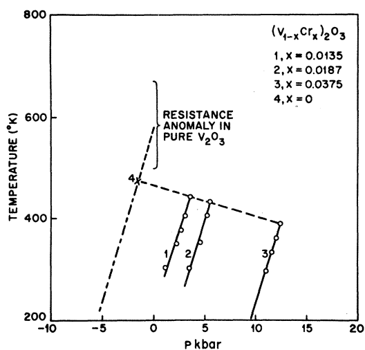
FIG. 3. M-I phase boundaries of three Cr-doped V_2O_3 samples (solid line). The dotted line in the negative pressure region (experimentally unrealizable) is for pure V_2O_3 and has been drawn parallel to the solid lines. The critical point ( x ) for V_2O_3 (obtained by extrapolation) has P_c = -1.5 kbar and T_c = 474 °K. The extrapolated dashed line beyond the critical point intersects the temperature axis in the region where the high-temperature resistance anomaly in V_2O_3 is observed.
