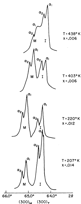
FIG. 5. X-ray powder diffraction line profiles of the (300) reflections from the metal (M) and insulator (I) phases of Cr-doped \text{V}_2\text{O}_3 . The twin peaks are from \text{CuK}\alpha_1 and \text{CuK}\alpha_2 radiation.
