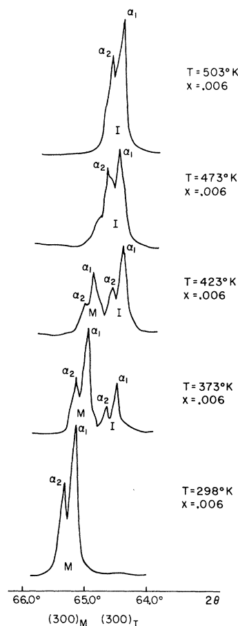
FIG. 6. X-ray powder diffraction line profiles for the (300) reflection from a 0.6% Cr-doped \text{V}_2\text{O}_3 . The (M) peak shifts more rapidly to smaller 2\theta with temperature compared to the (I) peak.
