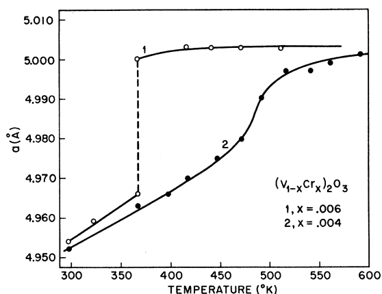
FIG. 7. Change in the lattice constant ( a ) for two Cr-doped V_2O_3 samples as a function of temperature. The sample with x = 0.006 exhibits a discontinuous jump. Sample with x = 0.004 shows a continuous and smooth but somewhat anomalous variation. The former is characteristic of subcritical and the latter of supercritical behavior.
