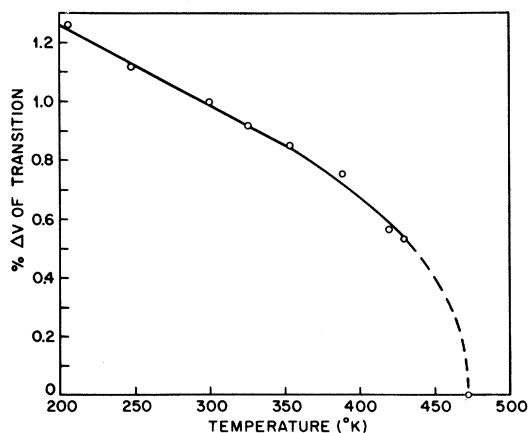
FIG. 8. Percent volume change along the M-I transition boundary obtained from x-ray data at atmospheric pressure, using samples with different Cr concentration. The \Delta V of transition was evaluated at the temperature where the separate (M) and (I) peaks were approximately equal in intensity. Some intermediate data points obtained at other temperatures are also included.
