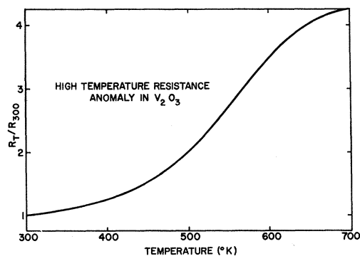
FIG. 4. High-temperature anomaly in pure V_2O_3 , from the data of Feinlieb and Paul (Ref. 3).
