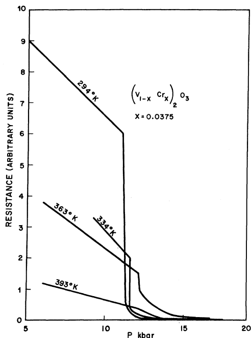
FIG. 1. Resistance-pressure isotherms for Cr-doped V_2O_3 .
