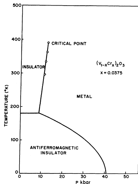
FIG. 2. Phase diagram of Cr-doped V_2O_3 containing 3.75-at.% Cr. The I and M phases have the corundum structure and the AF insulator is monoclinic.
